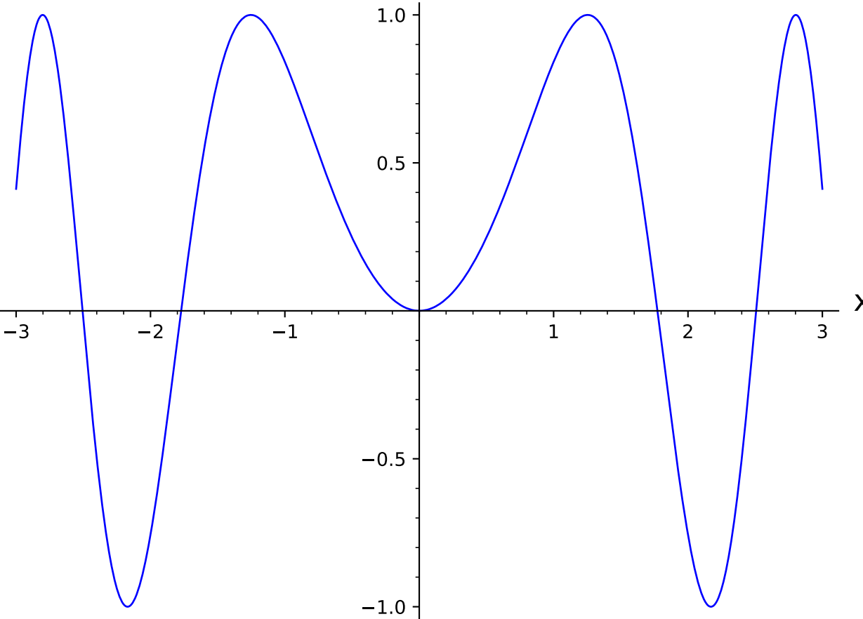
Plot of \sin(x^2)
